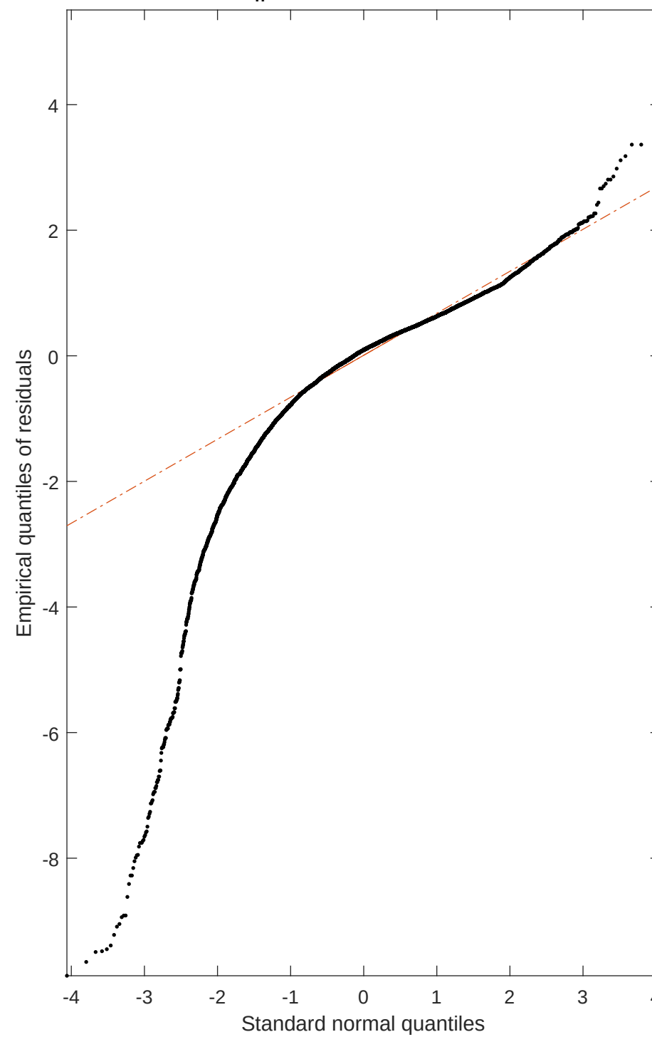
rel h um|temp: resid QQ-plot
