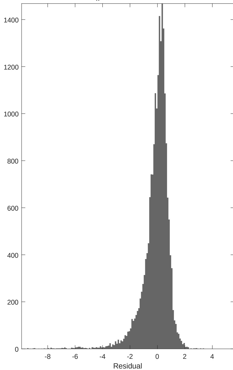
rel h um|temp: resid hist
